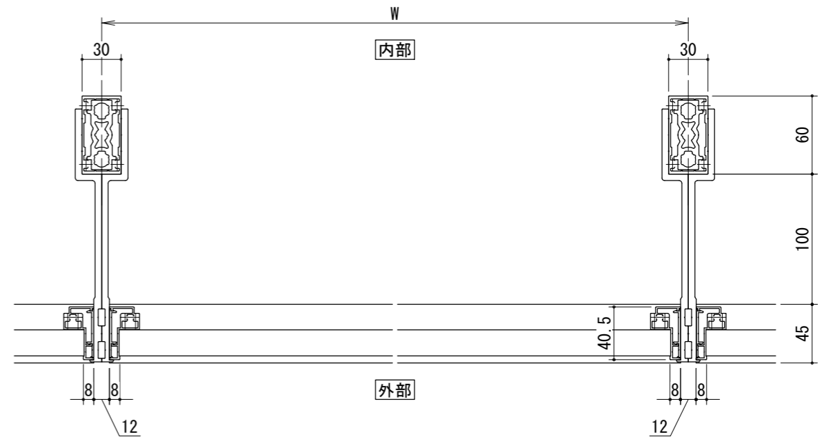
[30×60支柱]
