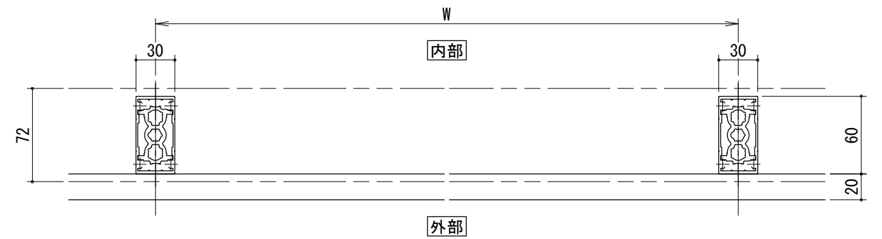
[30×60支柱]
