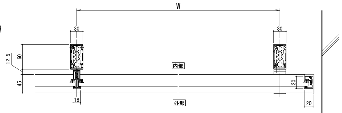
[30x60支柱]
